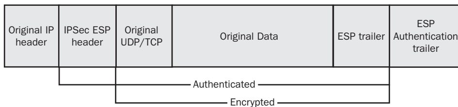
Figure 8.1 Transport mode IPSec
