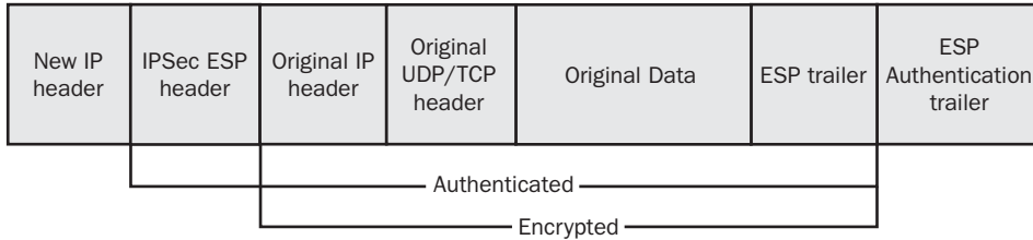
Figure 8.3 Tunnel mode IPSec
